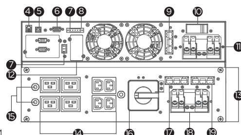
OLS5KERT5UM/OLS6KERT5UM/OLS8KERT5UM/OLS10KERT5UM
